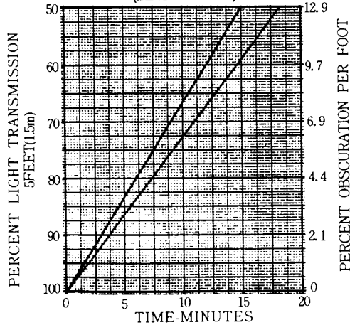
FIGURE 4 SMOKE BUILD-UP RATE-SENSITIVITY TEST (BLACK SMOKE)
