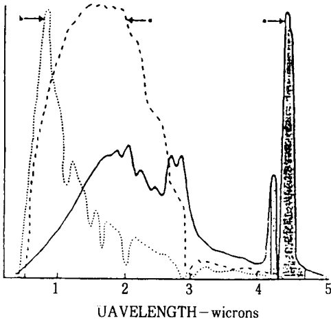
그림 4. Spectrums of a) Typical Carbonaceous Fire b) Solar Radiation at Ground Level c) Tungsten Filament Lamp
