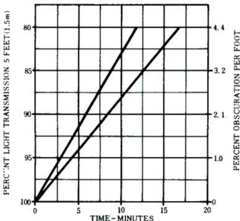
FIGURE 2 SMOKE BUILD-UP RATE - SENSIVITY TEST GRAY SMOKE - COTTON WICK - 30fpm
