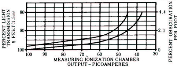
FIGURE 1 SENSIVITY TEST LIMITS GRAY SMOKE - COTTON WICK - 30fpm
