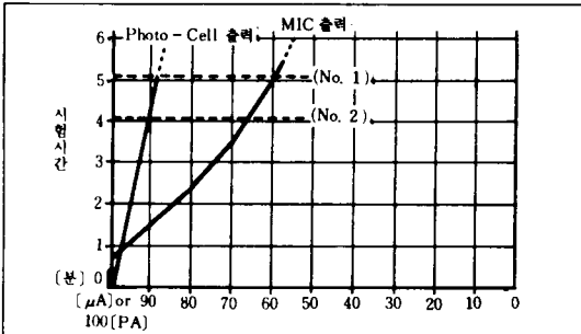
광속전달율 (Percent Light Transmission) 및 MIC 출력
