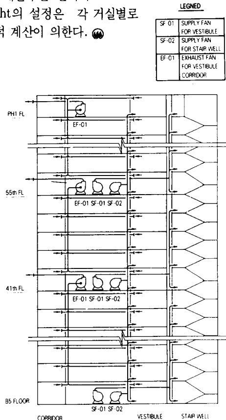
(SMOKE CONTROL SYSTEM PIPE SCHEMATIC)
